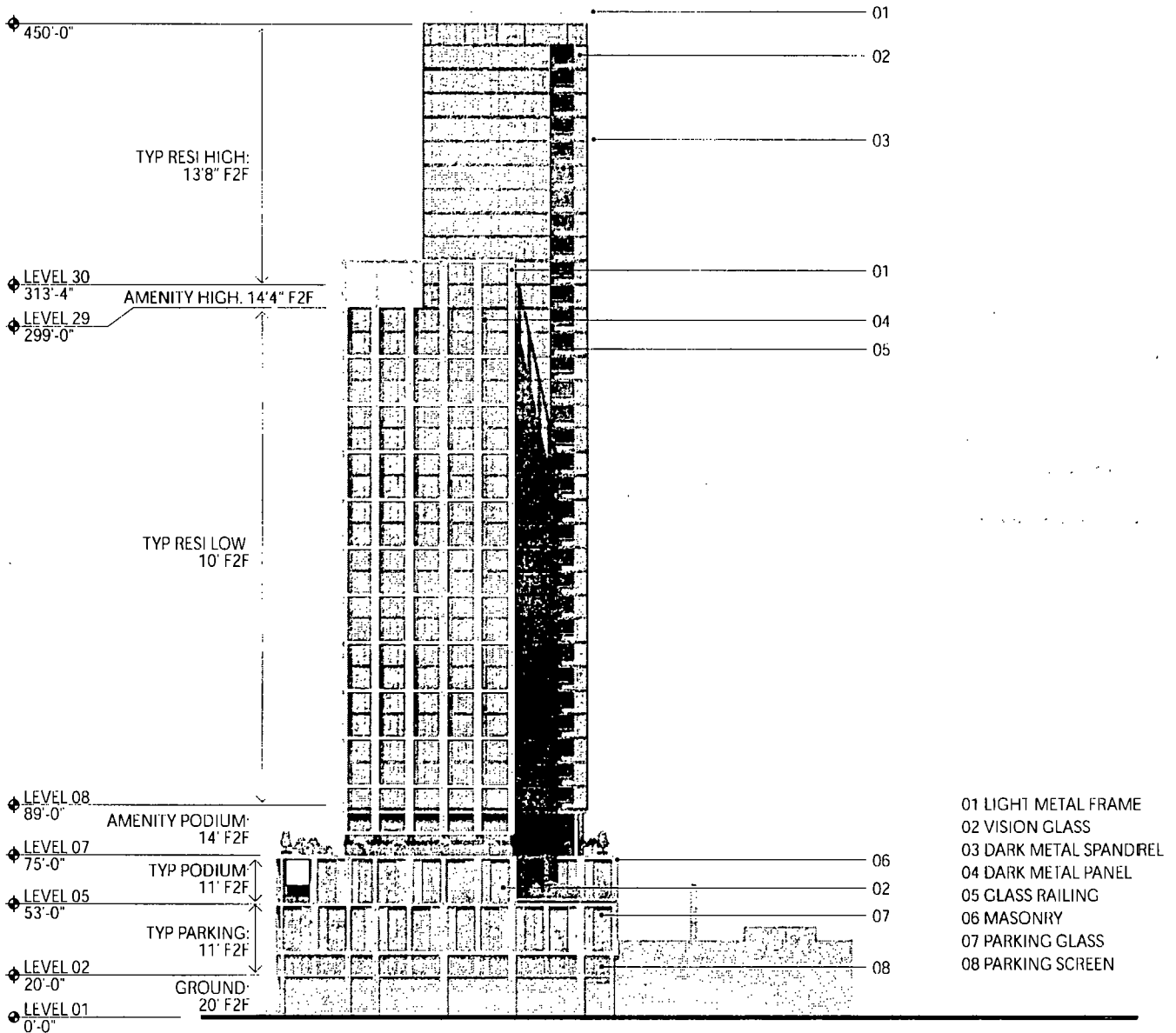
NORTH ELEVATION
