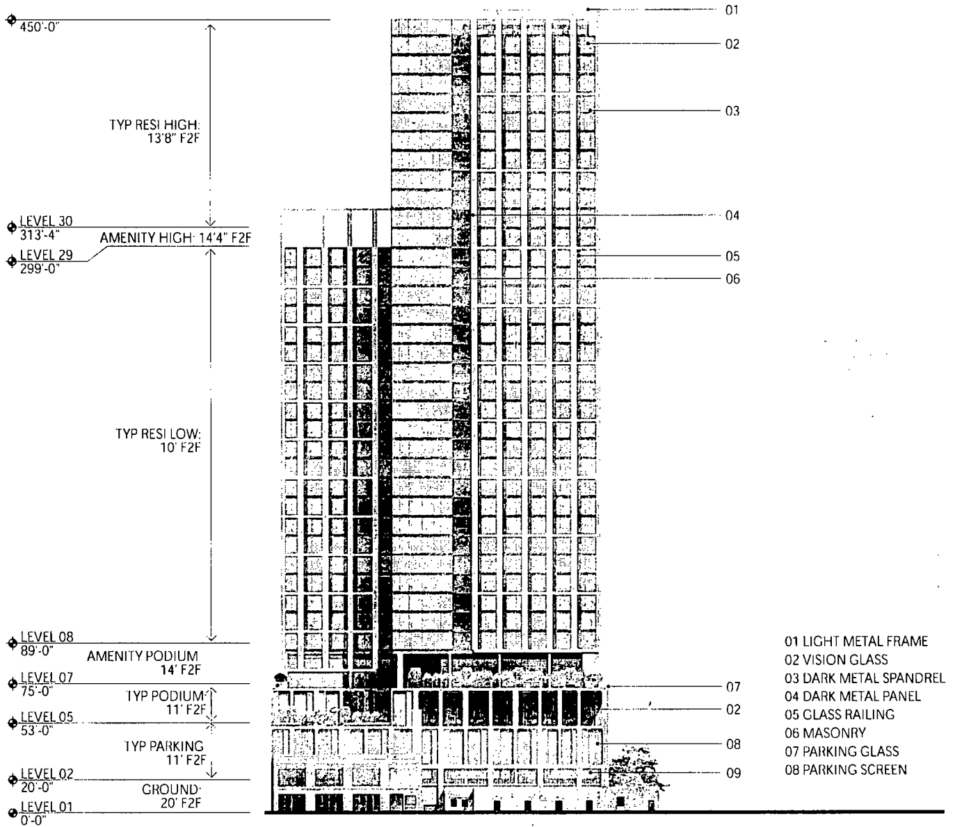
WEST ELEVATION
