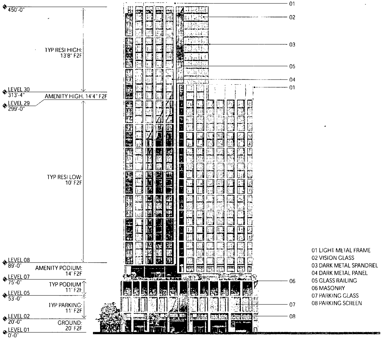
EAST ELEVATION
