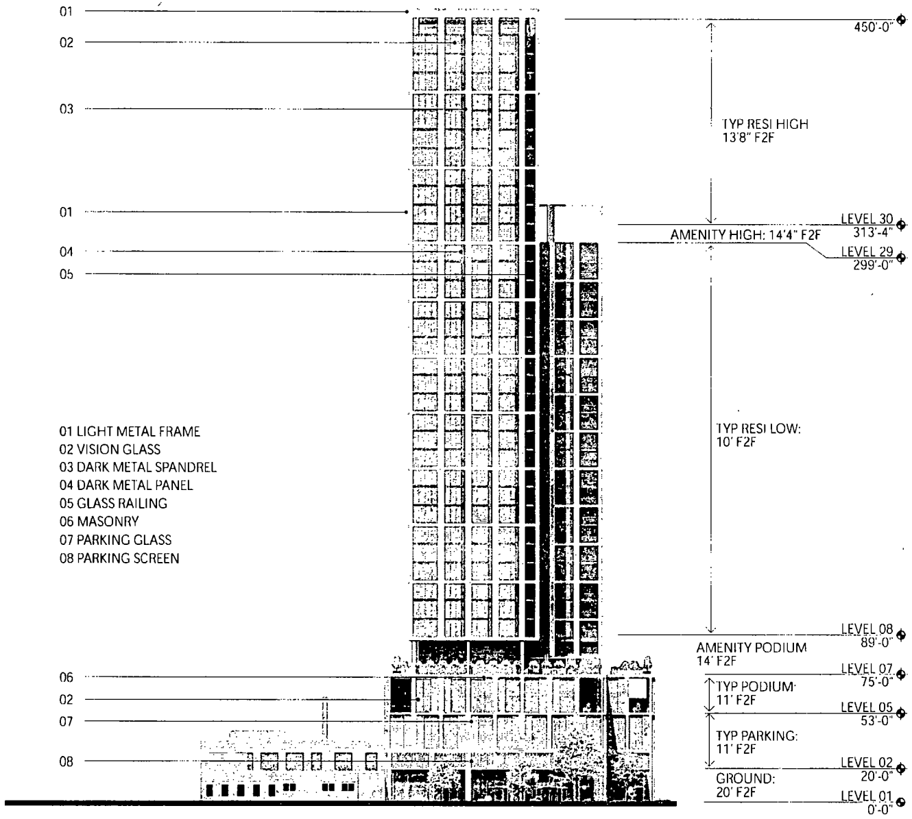
SOUTH ELEVATION
