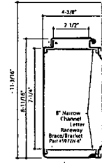
2 Piece 8" Narrow Channel Letter Raceway w/Raceway Cover Part #1981 & 1982N Part #1976N
