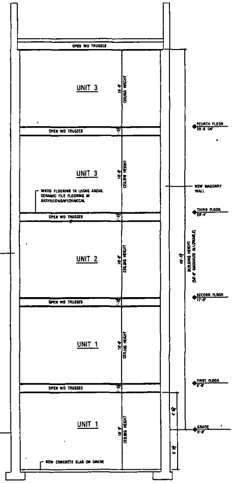
2 SCHEMATIC SECTION 1/8" = 1'-0"
