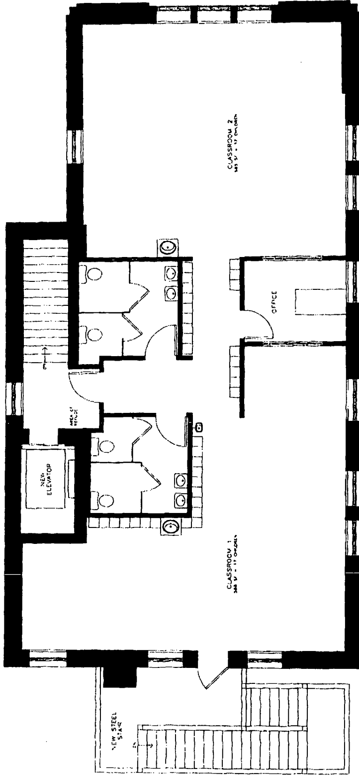
2ND FLOOR PLAN SCALE 1/4" = 1'-0" NORTH
