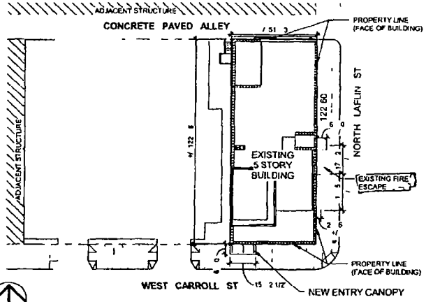
1 SITE PLAN
