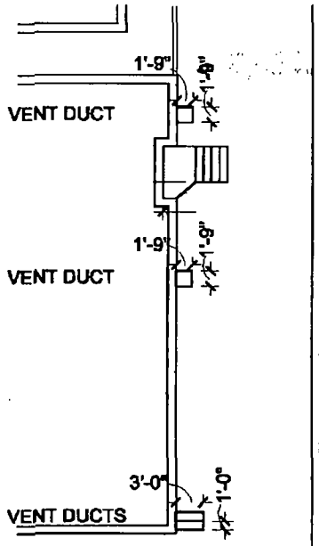
2 Dimensioned Site Plan SCALE 1/16"=1'-0"
