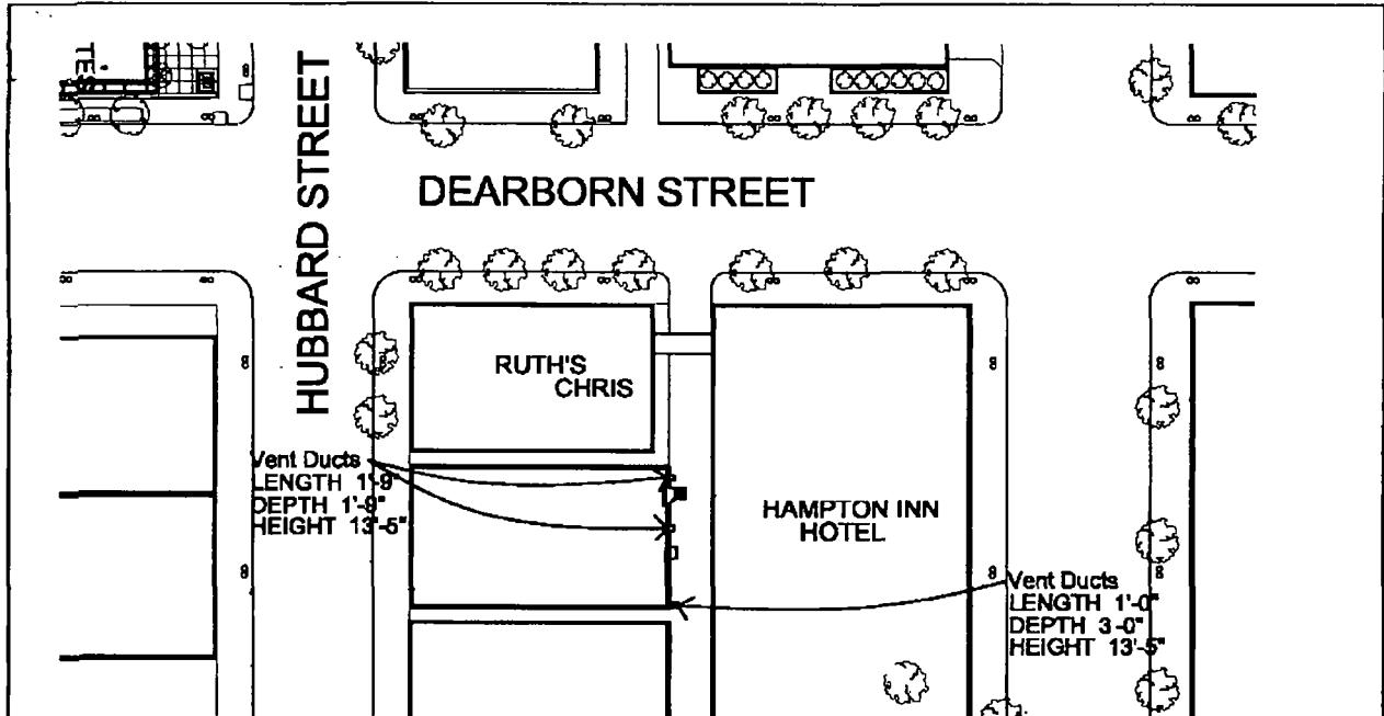
1 Site Plan of Vent Ducts SCALE 1/8"=1'-0"
