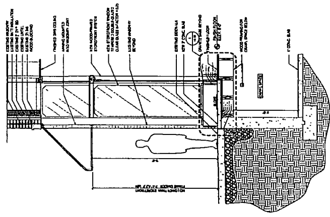
1 STOREFRONT SECTION 1/8\"/>
