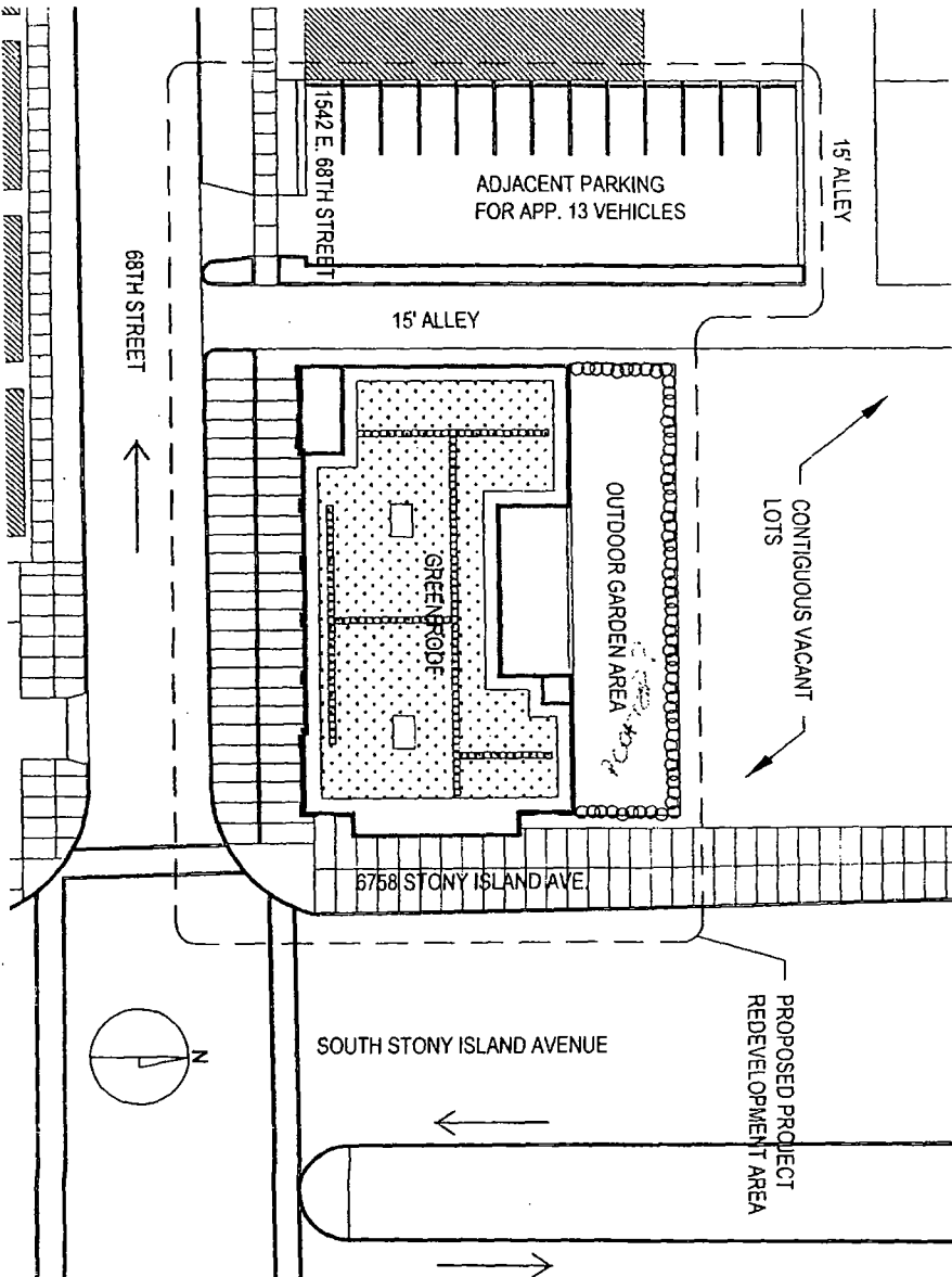
SITE PLAN - 1"=30'
