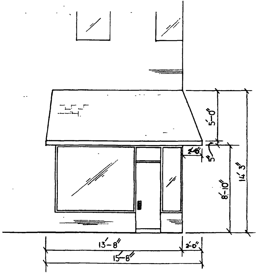
EAST ELEVATION
