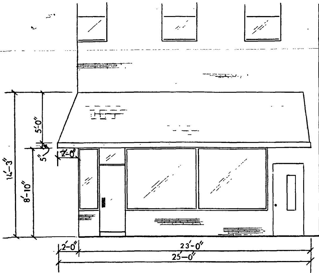
NORTH ELEVATION
