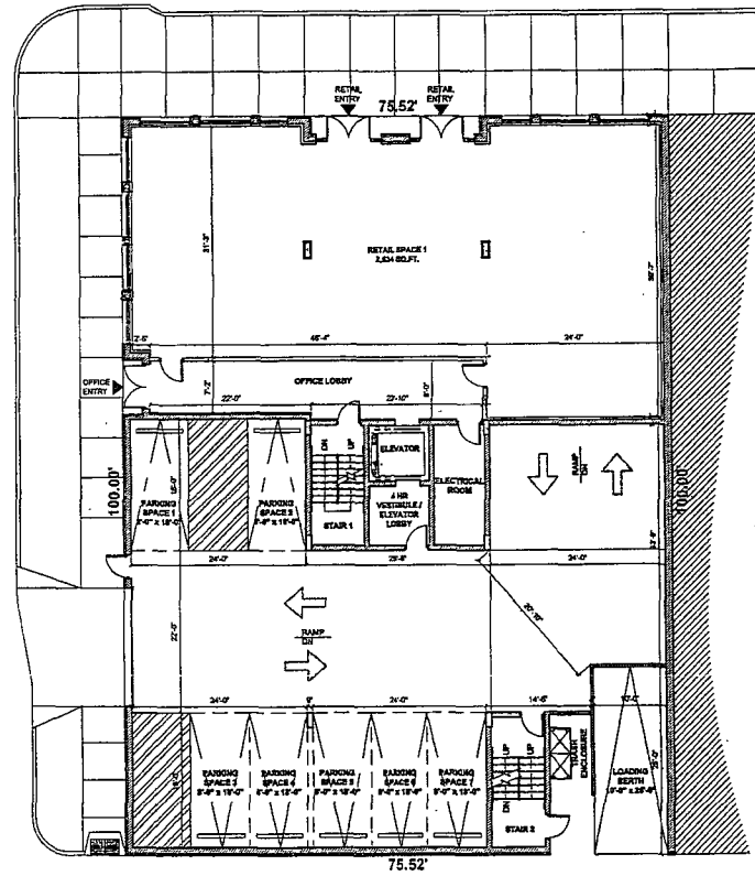
First Floor Plan Scale: 1/8"=1'-0"
