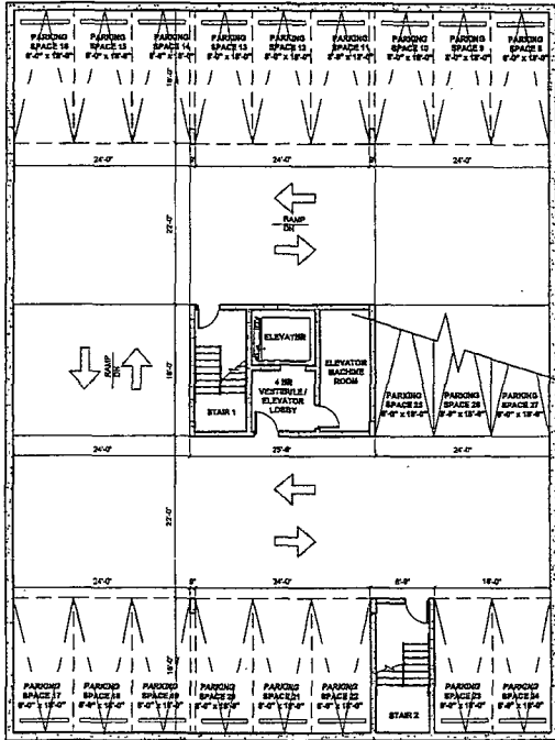
Basement / Garage Plan Scale: 1/8"=1'-0"
