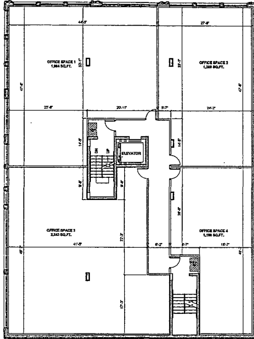
Third - Fifth Floor Plan
