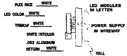
CHANNEL LETTER CROSS-SECTION
