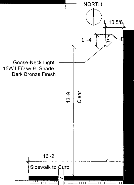
CLARK ST ELEVATION SCALE 1/4 = 1-0
