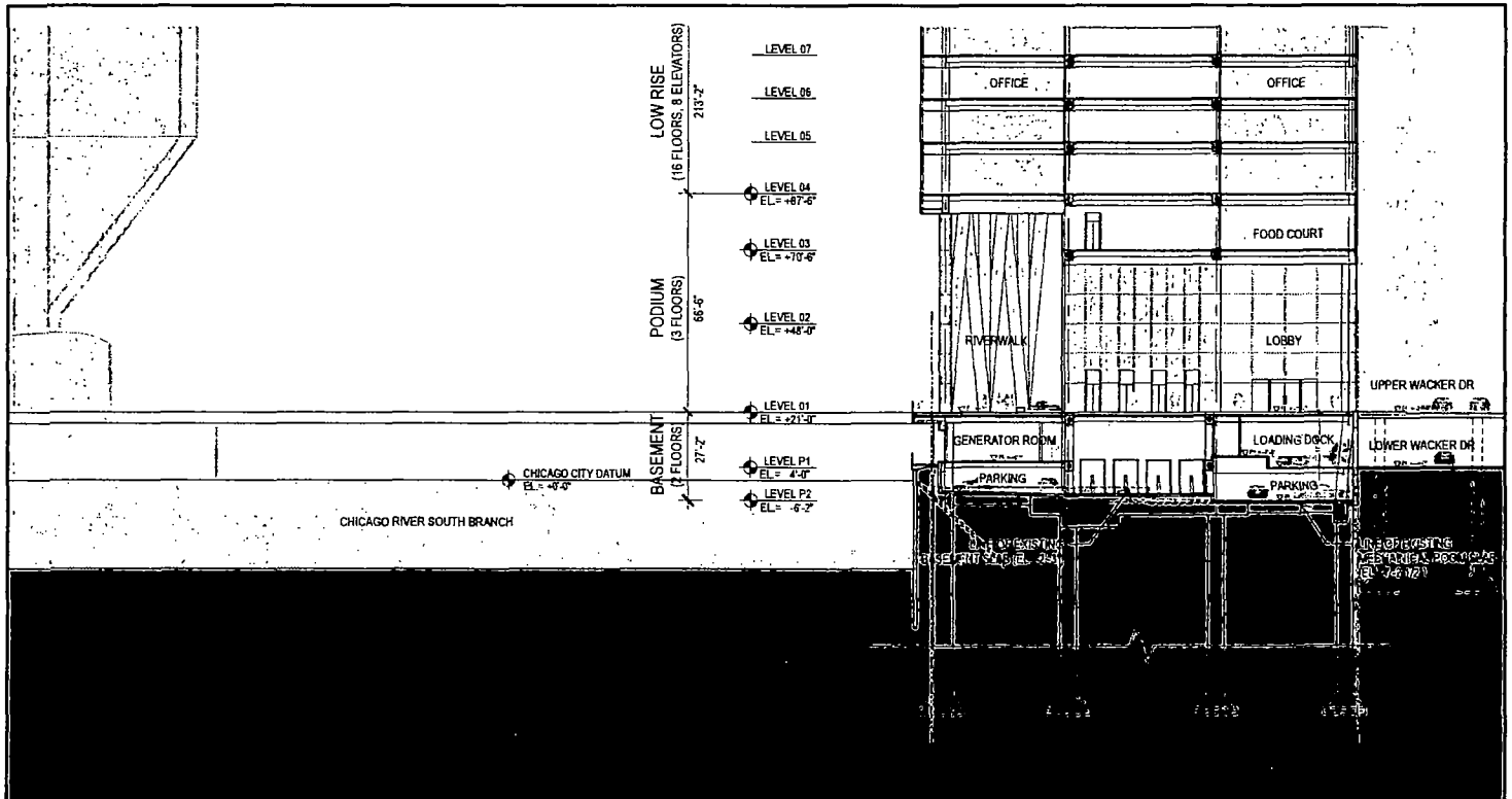
PODIUM ENLARGED SECTIONS 1 0 12' 25' 50' 75'
