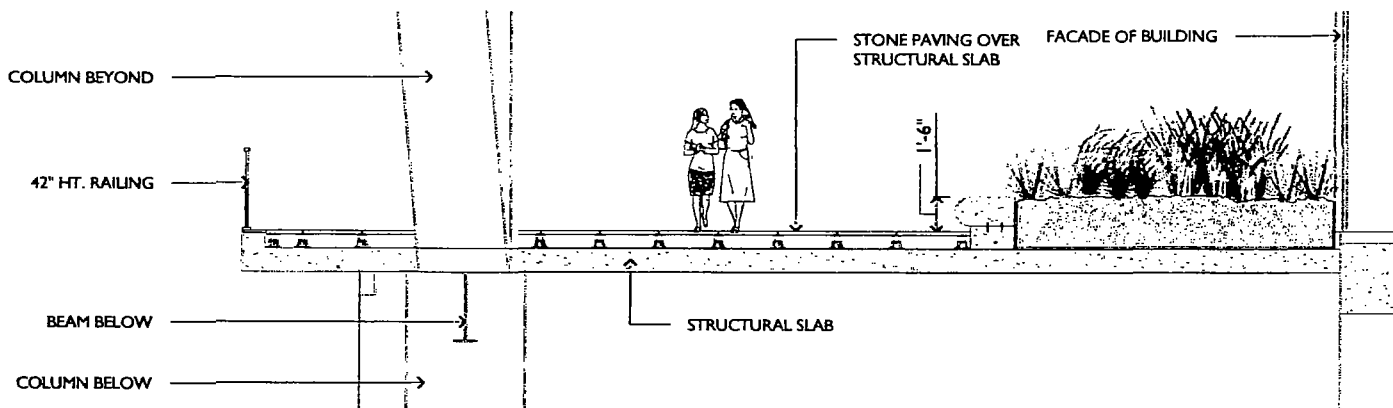
3 SECTION THROUGH RIVER PROMENADE SCALE: 1/8" = 1'-0"
