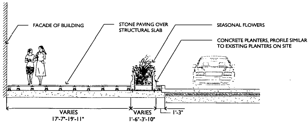
2 SECTION THROUGH PARKWAY PLANTER SCALE: 1/8" = 1'-0"
