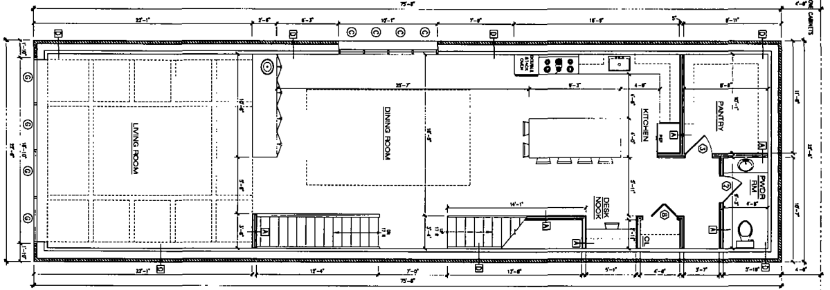
Proposed 2nd Floor Plan SCALE 1/4" = 1'-0"
