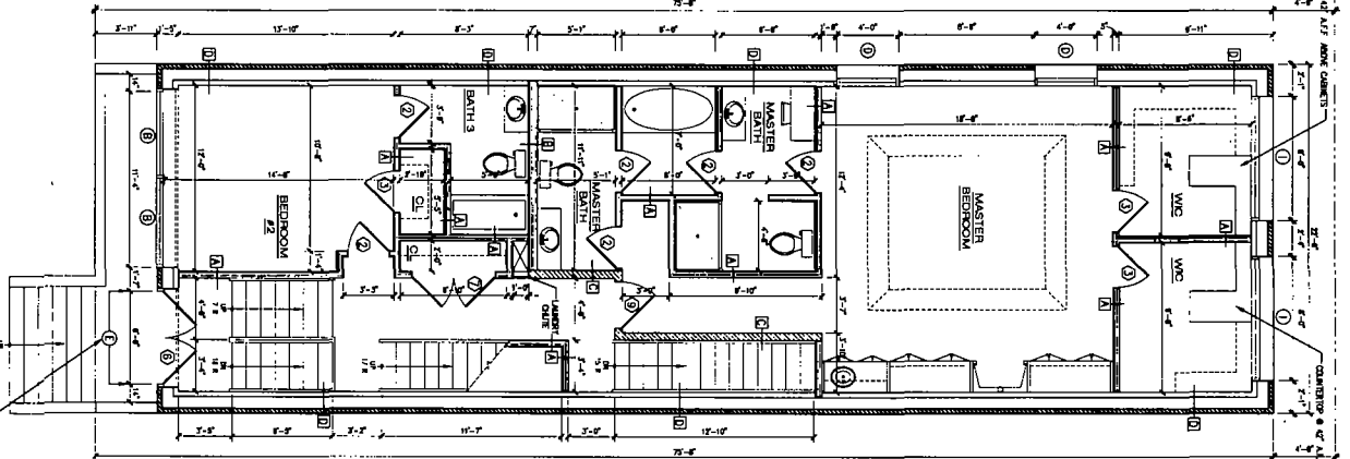
Proposed 1st Floor Plan SCALE 1/4" = 1'-0"
