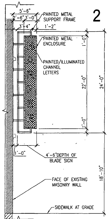
2 SECT THRU EAST WALL SCALE 1/2" = 1'-0"
