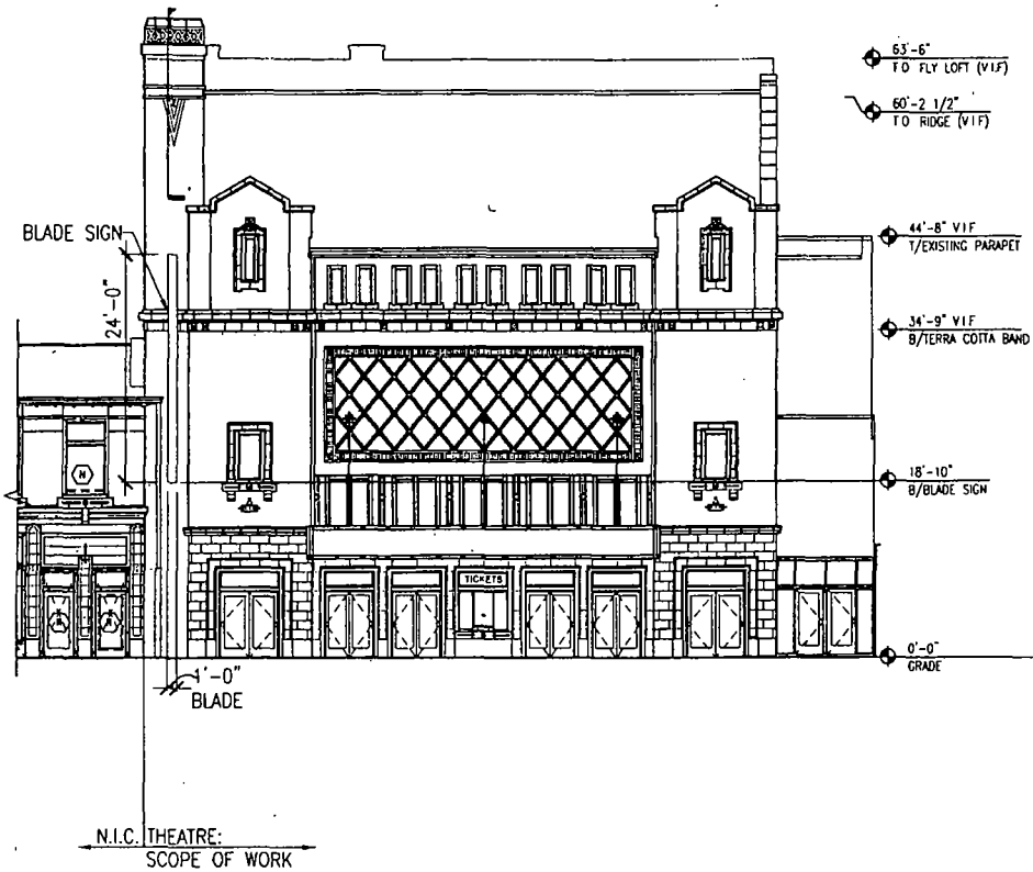
1 EAST ELEVATION SCALE 1/16" = 1'-0"
