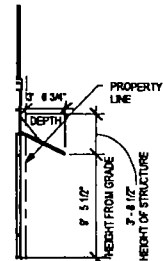
④ RETAIL CANOPY TYPICAL SECTION 1/8" = 1'-0"
