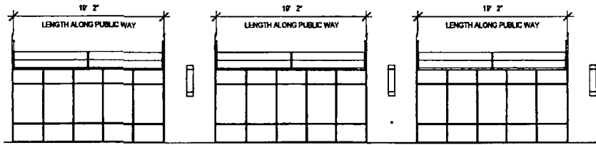
② SHERIDAN CANOPY ELEVATION 1/8" = 1'-0"
