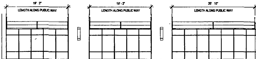
③ SHERIDAN CANOPY ELEVATION CONTINUED 1/8" = 1'-0"
