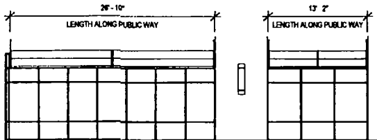
① ALBION CANOPY ELEVATION 1/8" = 1'-0"
