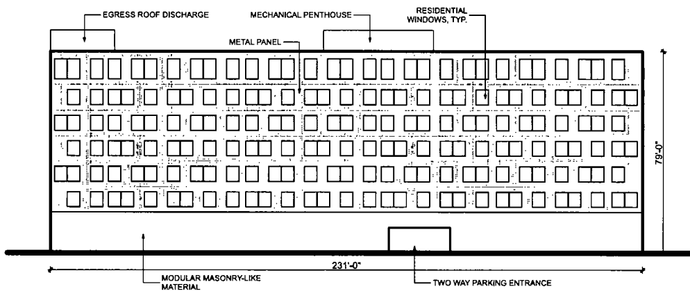
4 Bldg G - North SCALE 1" = 50'
