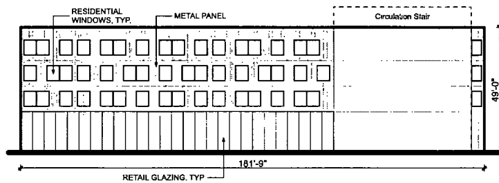
4 Bldg E - North SCALE: 1" = 50'
