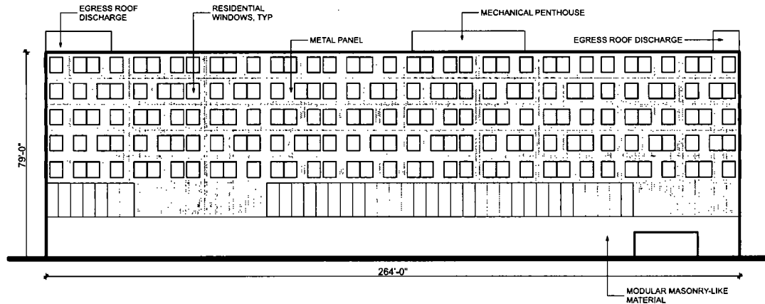
4 Bldg A - North SCALE: 1" = 50'
