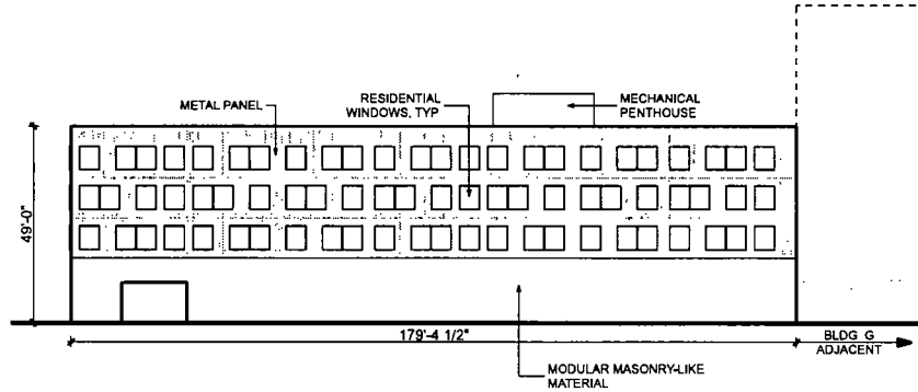
4 Bldg H - East SCALE: 1" = 50'
