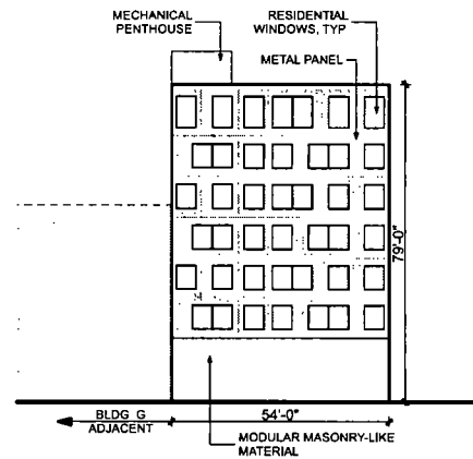
3 Bldg G - East SCALE 1" = 50'
