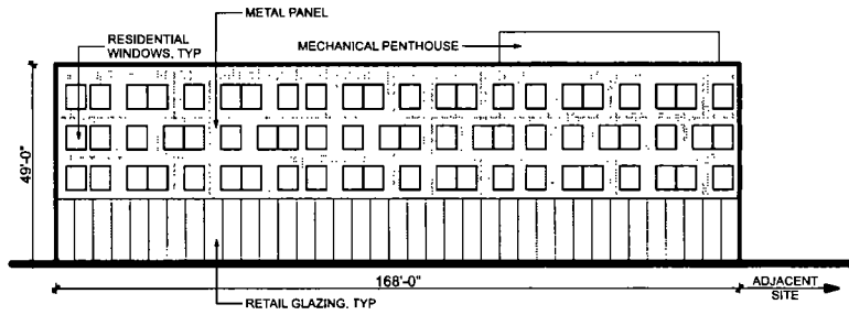
1 Bldg D - South SCALE 1" = 50'
