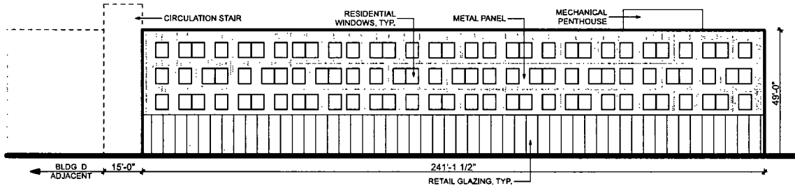
4 Bldg C - East SCALE 1" = 50'
