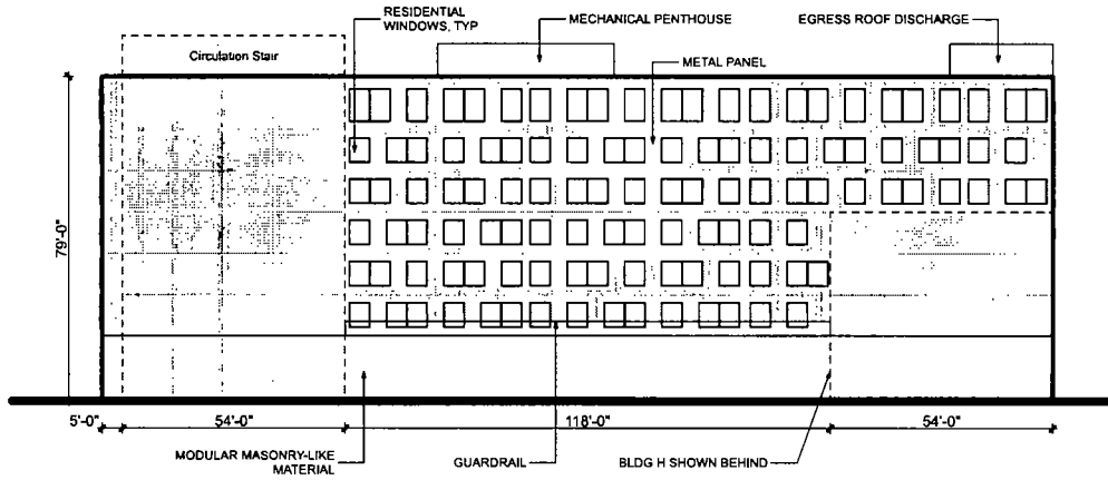
1 Bldg G - South SCALE 1" = 50'
