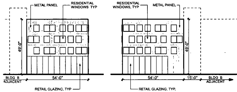
4 Bldg D - West SCALE 1" = 50'
