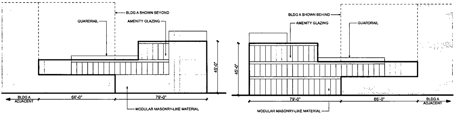
2 Bldg B - West SCALE 1" = 50'
