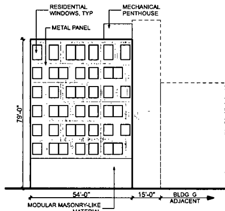
2 Bldg G - West SCALE 1" = 50'
