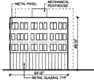
3 Bldg C - North SCALE 1" = 50'
