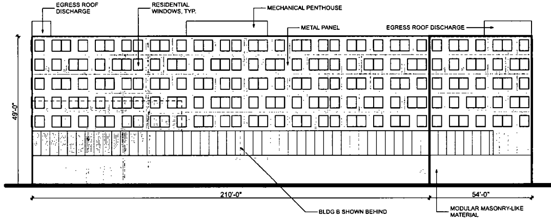
1 Bldg A - South SCALE 1" = 50'
