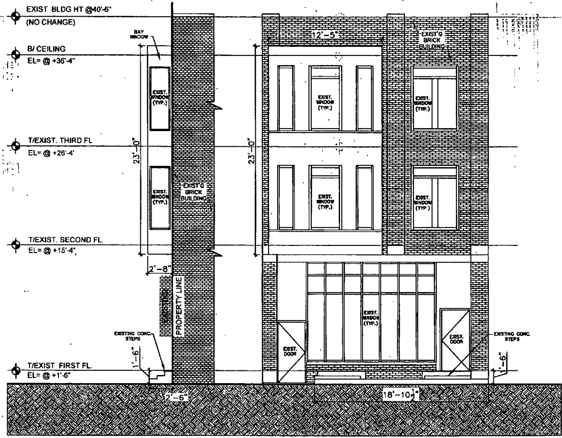
① SIDE ELEVATION W/ EXIST. CONC. STEPS/BAY WINDOW SCALE 1/8" = 1'-0"
