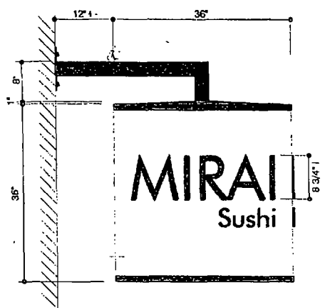
LED ILLUMINATED CUBE DISPLAY 3/4" = 1'-0"
