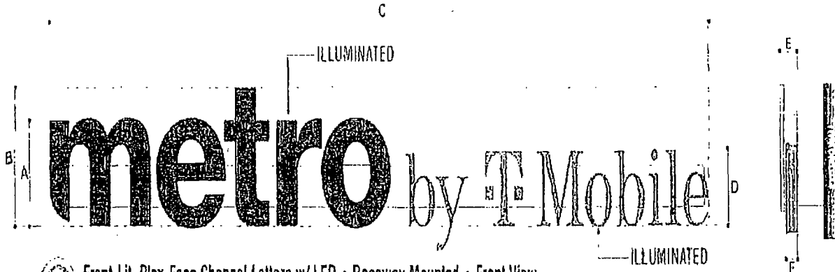
1.0 Front-Lit, Plex-Face Channel Letters w/ LED • Raceway Mounted • Front View • For Production / For Presentation
