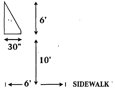
SIDE VIEW OF EXISTING AWNING
