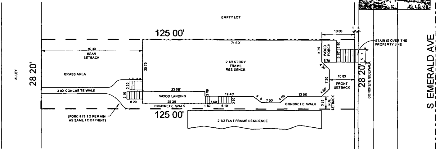
1 SITE PLAN 3/32 = 1'-0"
