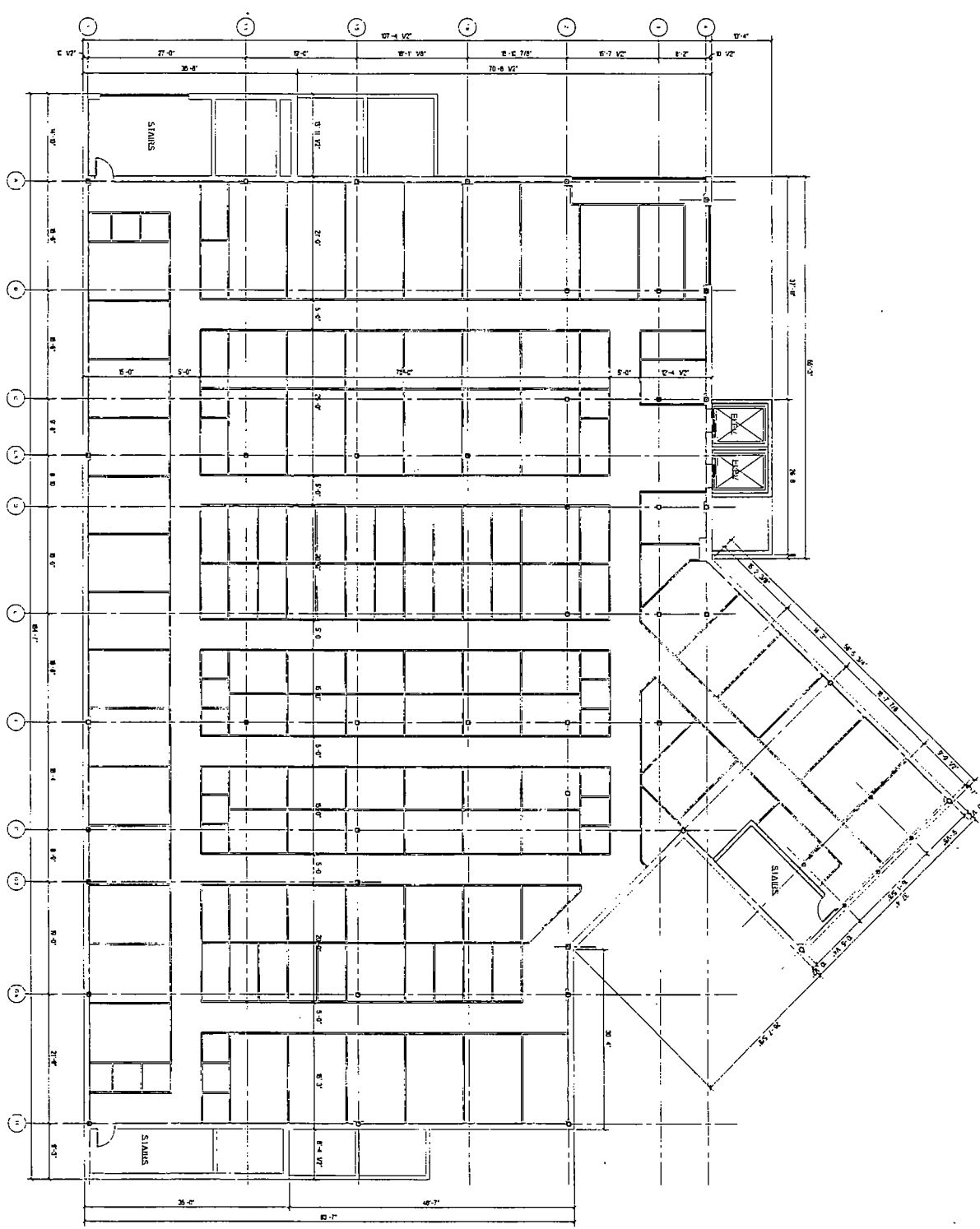
3rd Floor Plan SCALE: 1/8"=1'-0"
