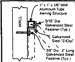
Enlarged Mounting Detail (Not To Scale)
