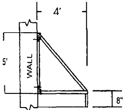
Side View of All Awnings (Closed Ended)
