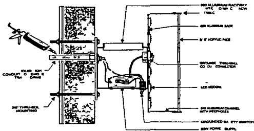
Typical U.L. Channel Letters with LEDs Mounted on Raceway Not to scale
