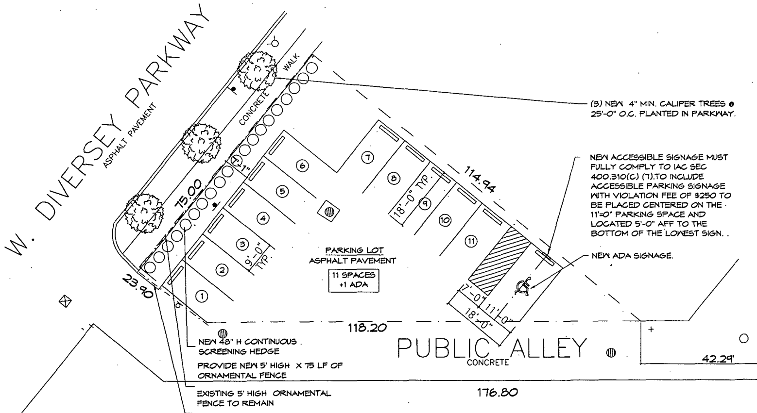
1 ENLARGED PARKING LOT SITE PLAN T-102 SCALE: 1/16" = 1' - 0"
