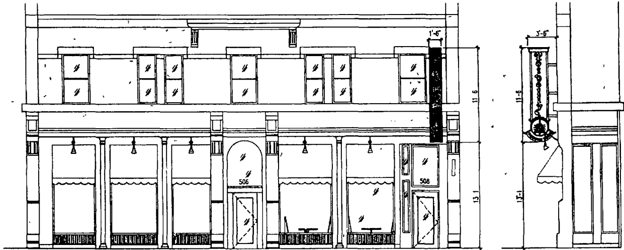
1 STOREFRONT ELEVATION 1/8" = 1'-0"
