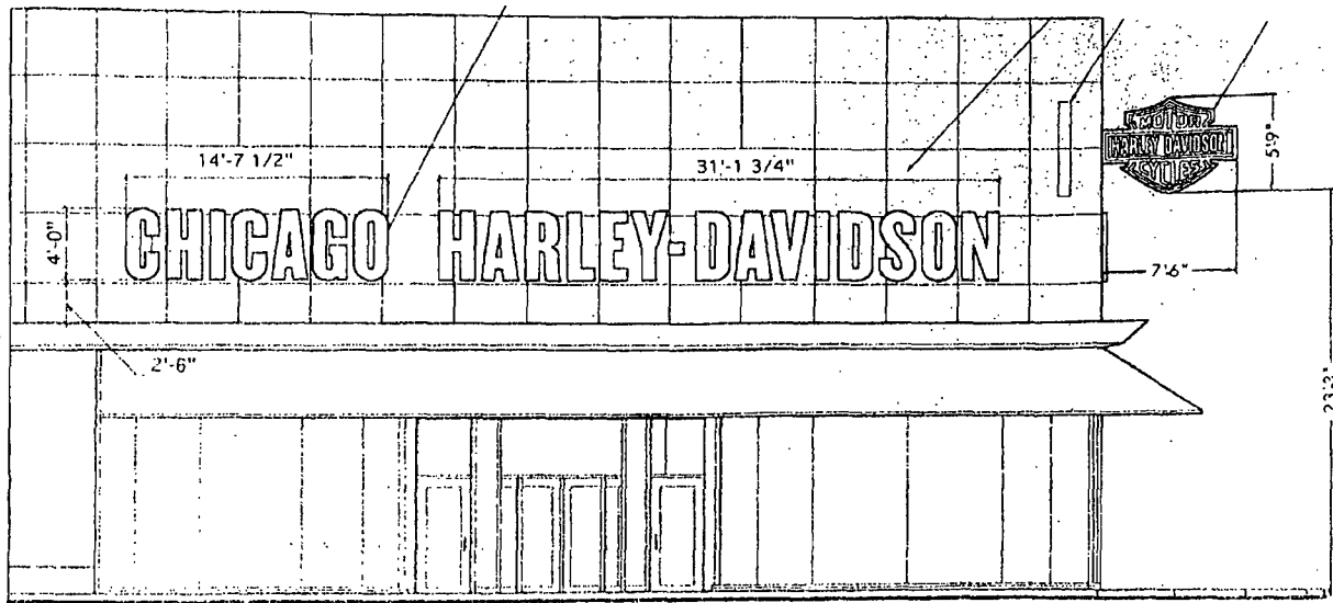
E02 Alt. A South Exterior Elevation (Ohio Street) Scale: 1/8" = 1'-0"
