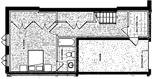
4 TYPICAL FLOOR BSMNT FLOOR PLAN 1/4" = 1'-0"
