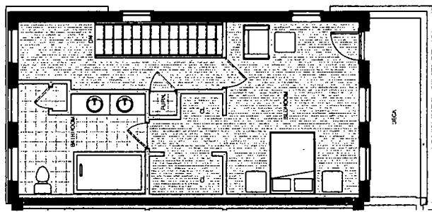
1 TYPICAL FLOOR 1ST FLOOR PLAN 1/4" = 1'-0"
