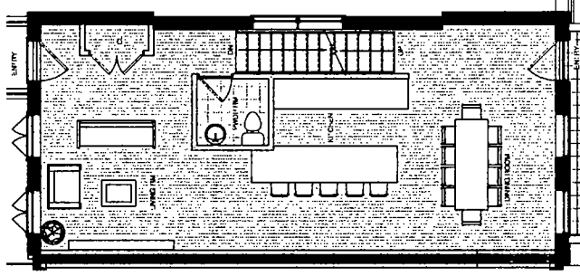
3 TYPICAL FLOOR 3RD FLOOR PLAN 1/4" = 1'-0"
