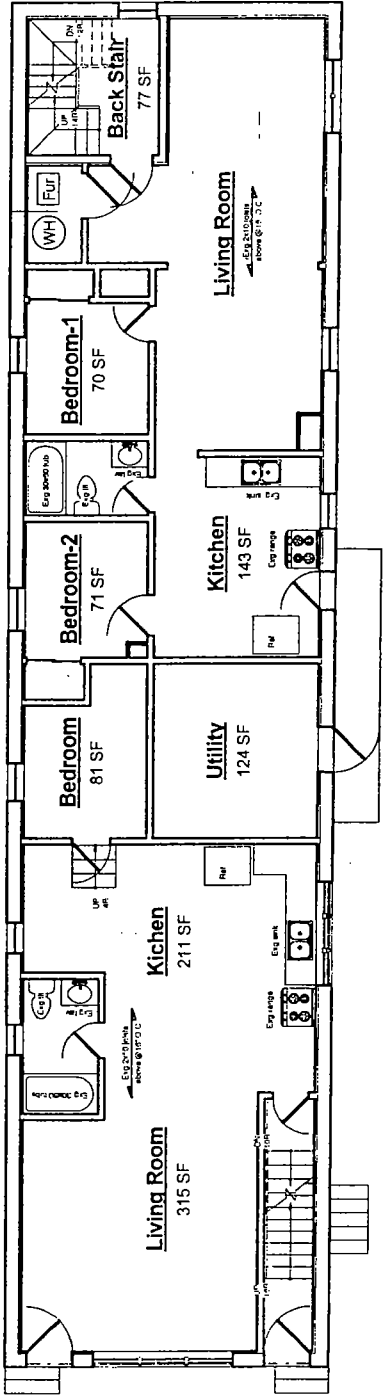
W N S E First Floor Plan Scale 1/8" = 1'-0"
