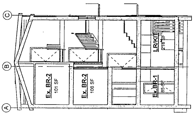
Section D-D Scale 1/8" = 1'-0"
