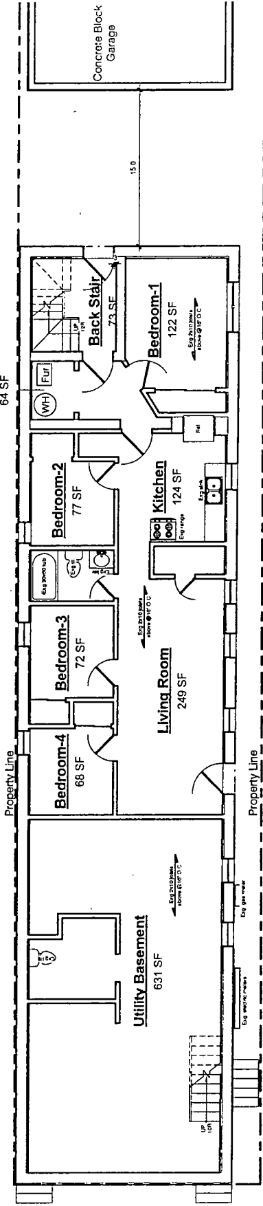
W N S E Basement Scale 1/8" = 1'-0"
