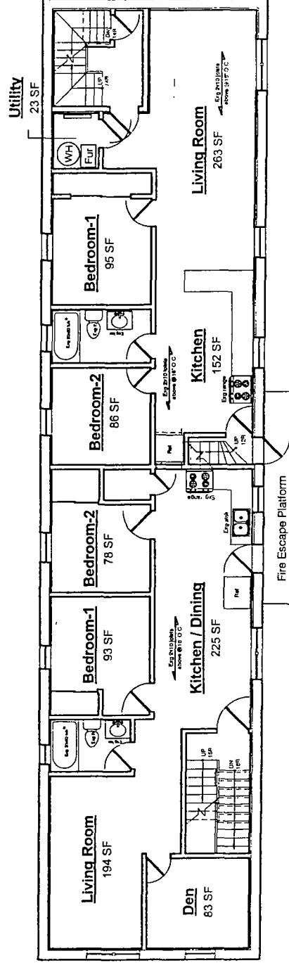
W N Second Floor Plan Scale 1/8" = 1'-0"
