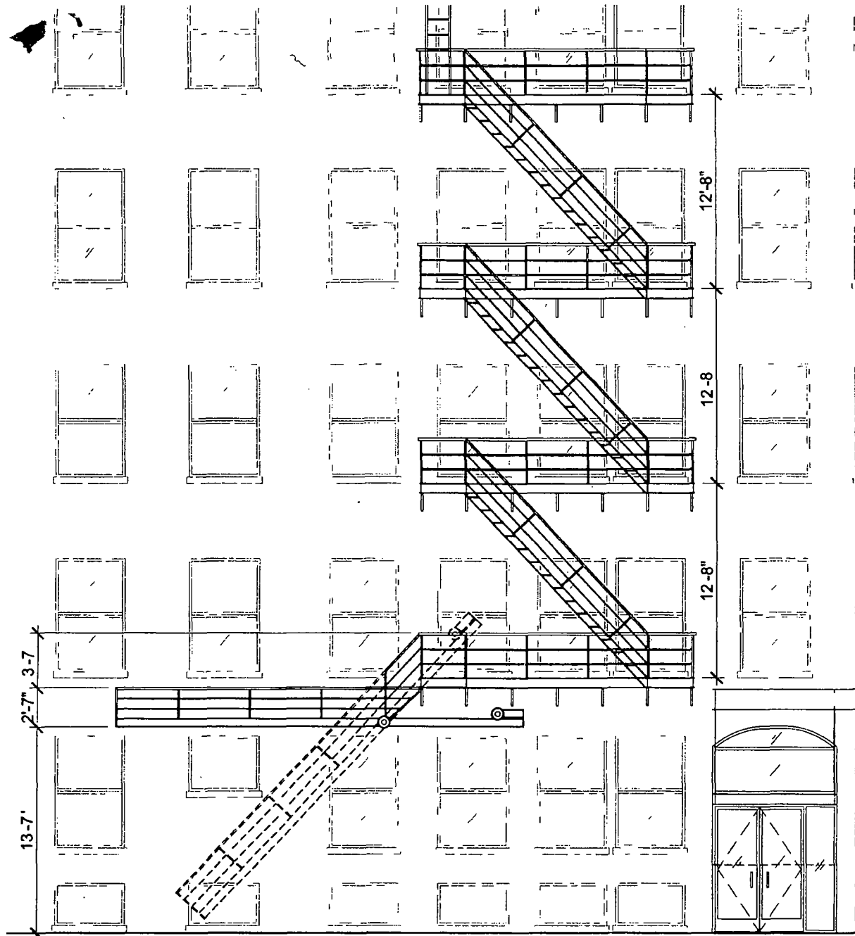
NORTH ELEVATION
