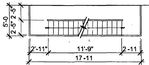
PLAN (TYPICAL FLOOR)
