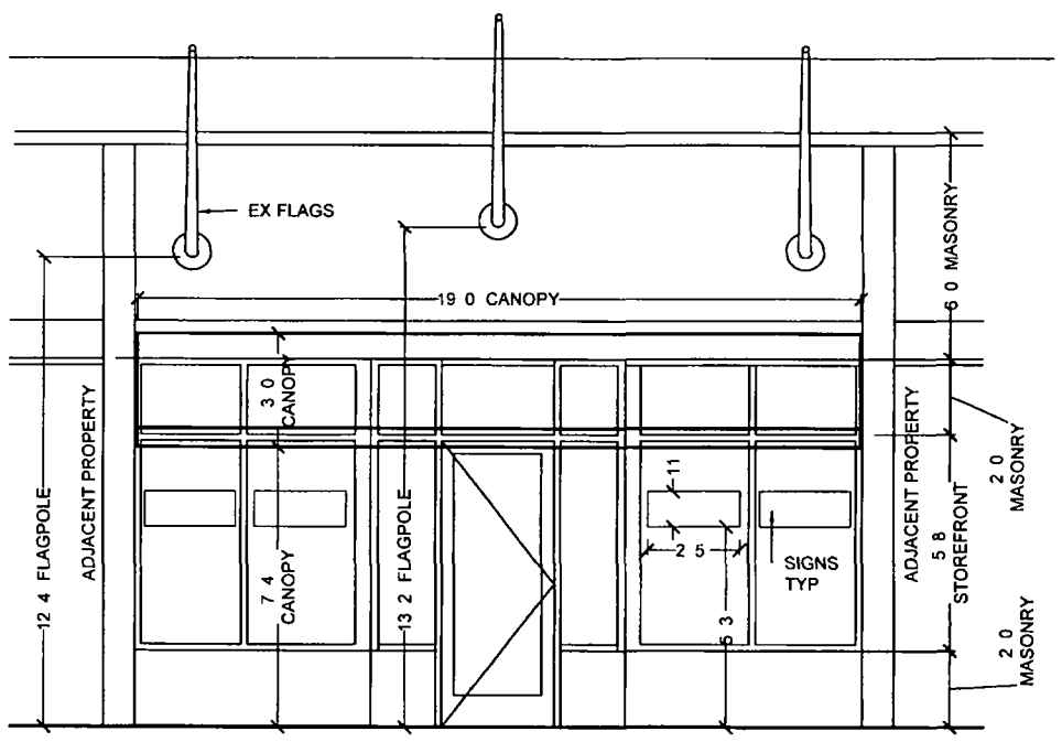
HALSTED WEST ENTRANCE ELEVATION A004
