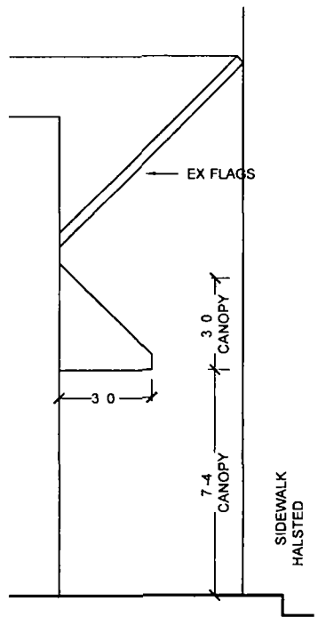
② SIDE VIEW LOOKING SOUTH 1/4" = 1'-0"
