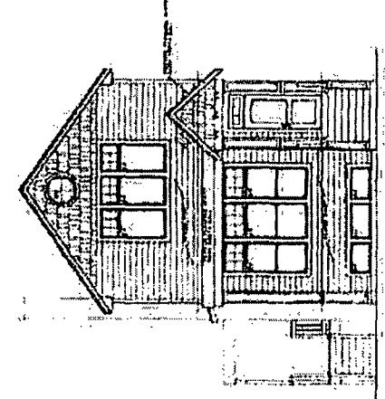
WEST ELEVATION 1/2" = 1'-0"
