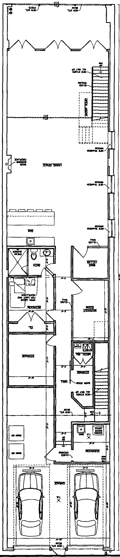
PROPOSED FIRST FLOOR PLAN SCALE: 1/8"=1'-0"
