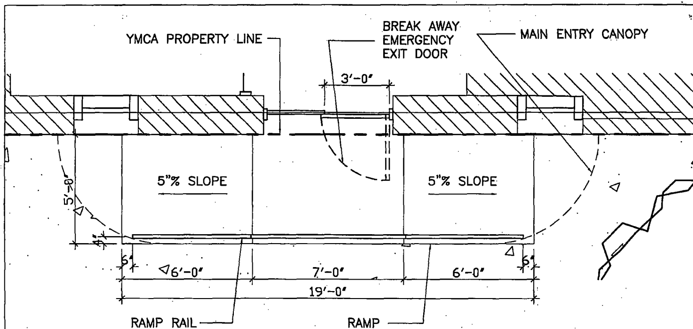
1 ACCESSIBLE RAMP AT MAIN ENTRY MARSHFIELD BUILDING PLAN
