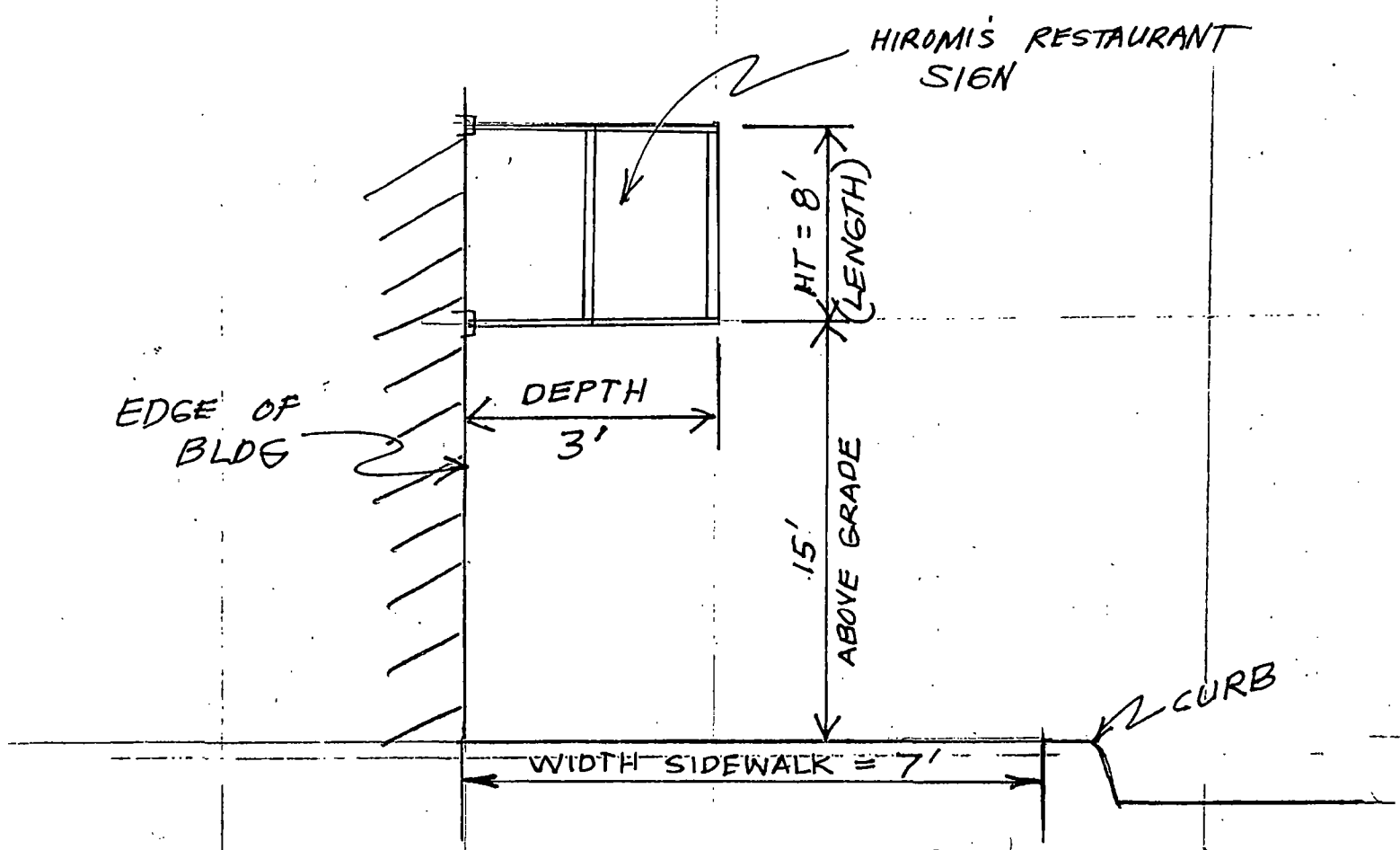
SIDE VIEW (LOOKING WEST)
