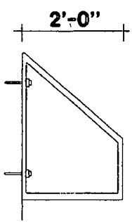
2' PROJECTION STEEL CLIPS WITH 3/8" EXPANSION BOLTS
