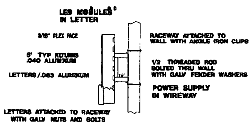
CHANNEL LETTER CROSS-SECTION
