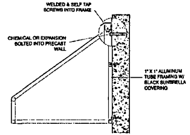
TYP. SECTION THRU AWNING DETAIL
