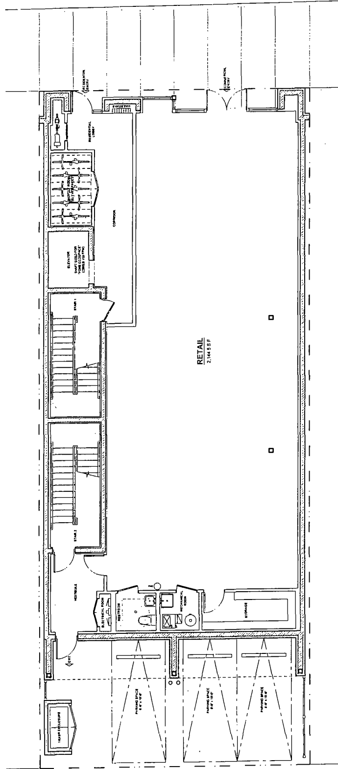
1 FIRST FLOOR PLAN P11 1/8" = 1'-0"
