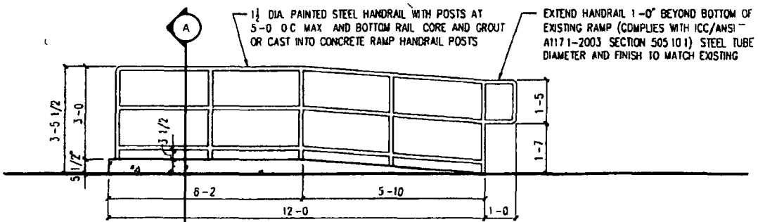
3 RAMP ELEVATION SCALE 1/4" = 1'-0"
