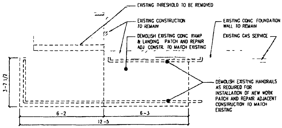
1 DEMOLITION PLAN SCALE 1/4" = 1'-0"
