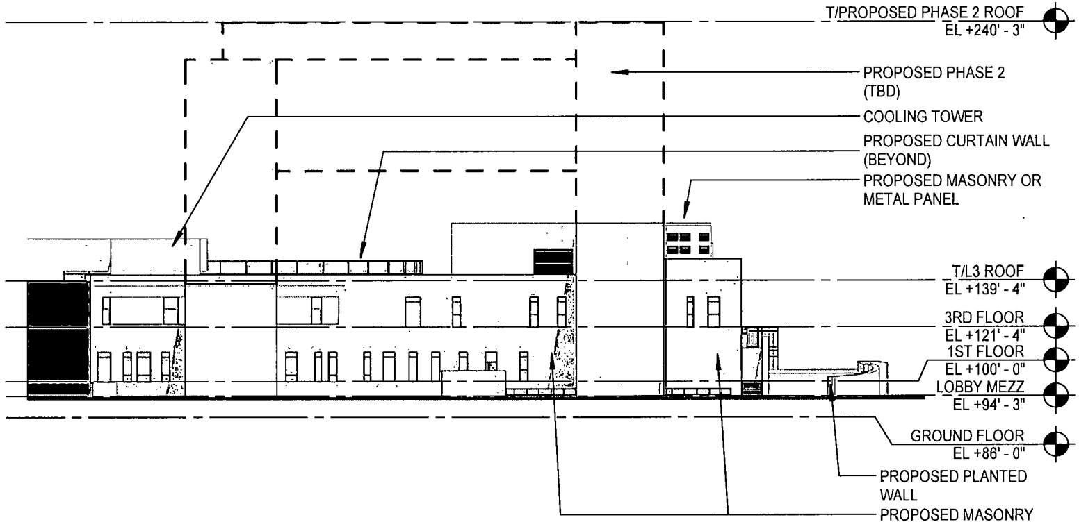
1 EAST ELEVATION - Phase 1 SCALE: 1" = 50'-0"
