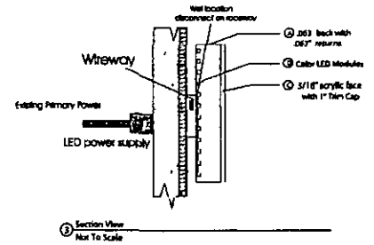
Typical Raceway Mount channel Letters with LED's
