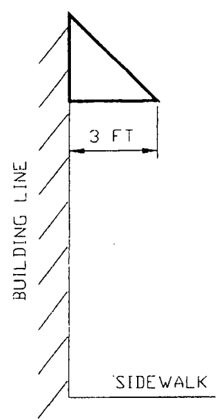
DEPTH OF CANOPY OVER PUBLIC WAY
