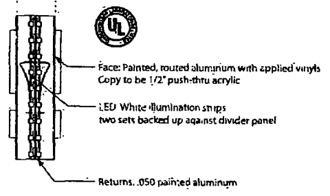
2. Double Face Blade Sign - LED Lighting TYPICAL - Section Detail
