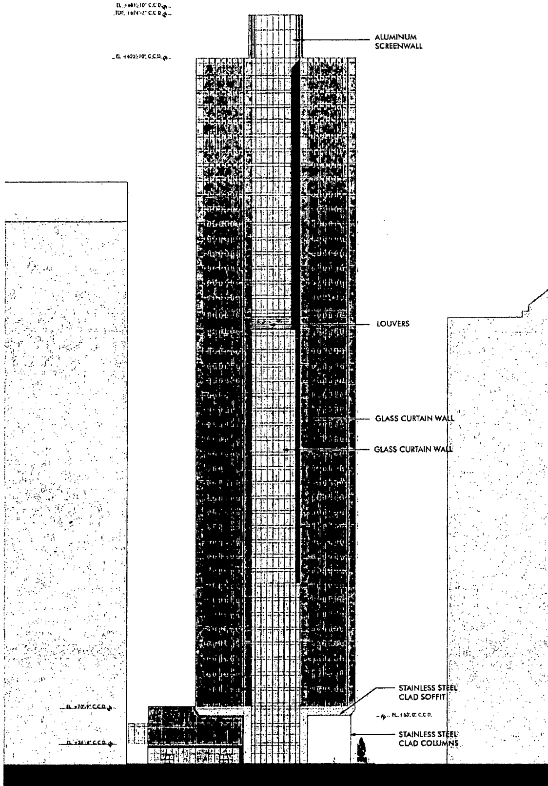
BUILDING ELEVATION - WEST
