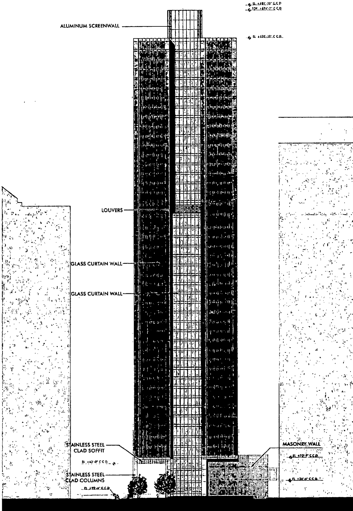
BUILDING ELEVATION - EAST
