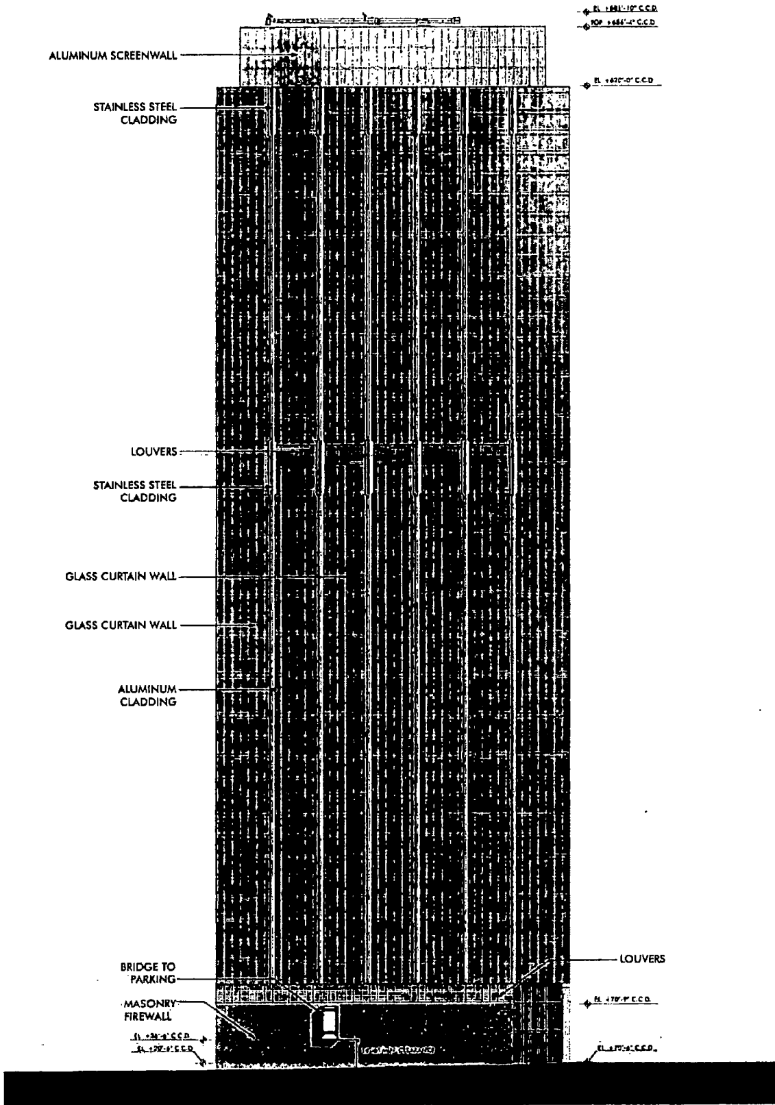
BUILDING ELEVATION - NORTH
