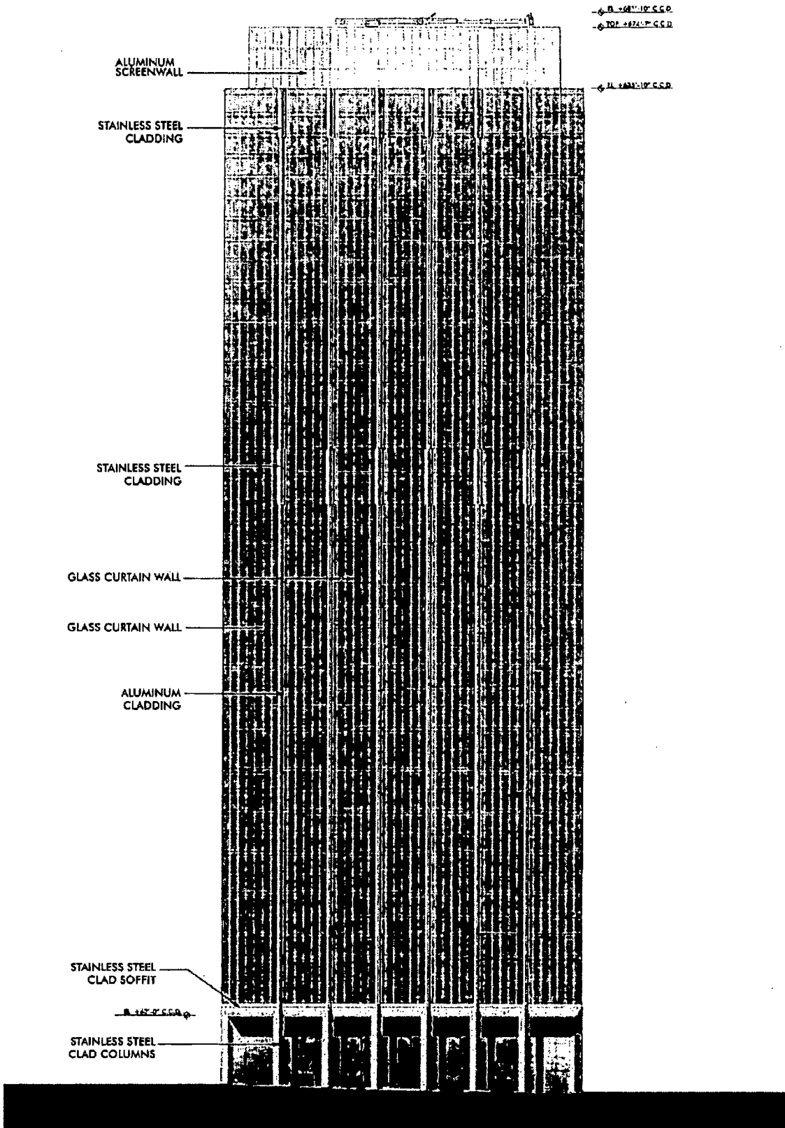
BUILDING ELEVATION - SOUTH
