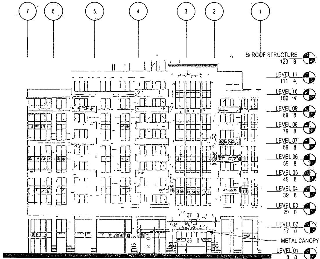
EAST ELEVATION
