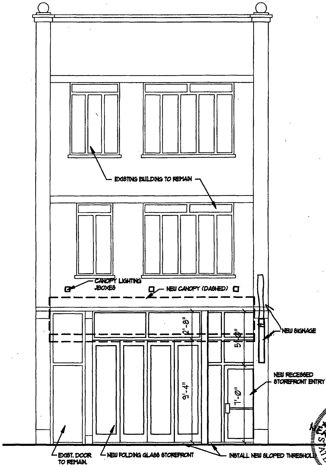
4 PROPOSED FRONT (SOUTH) ELEVATION A-2
