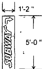
Directional Banner on Ohio State St. Elevation.
