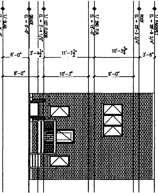
1 TYPICAL NORTH ELEVATION A2.1 1/4"=1'-0"
