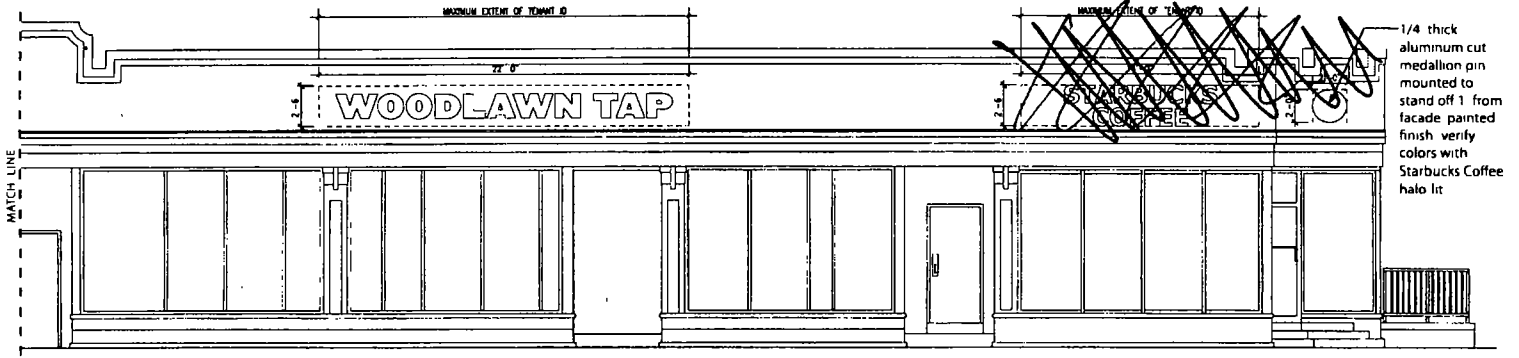
SOUTH (FRONT) ELEVATION 3/16 = 1/8"
